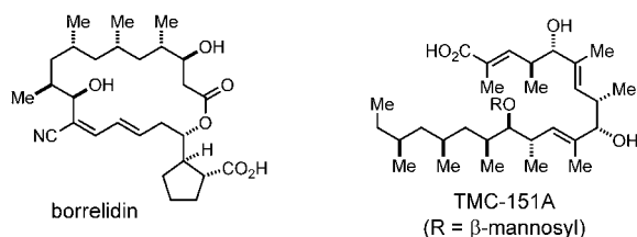
Scheme 1. Representative deoxypropionate-containing natural products.
