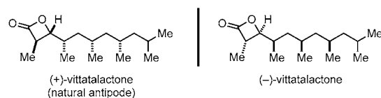
B) A concise convergent synthesis of (–)-vittatalactone
