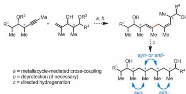
Scheme 2. A convergent strategy for deoxypropionate synthesis.
