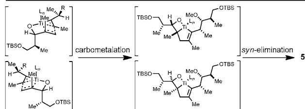
Scheme 3. Reductive cross-coupling process.
