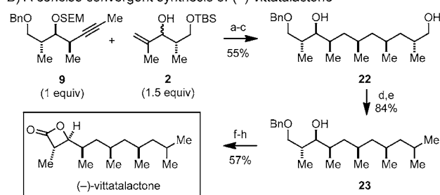
B) A concise convergent synthesis of (–)-vittatalactone
